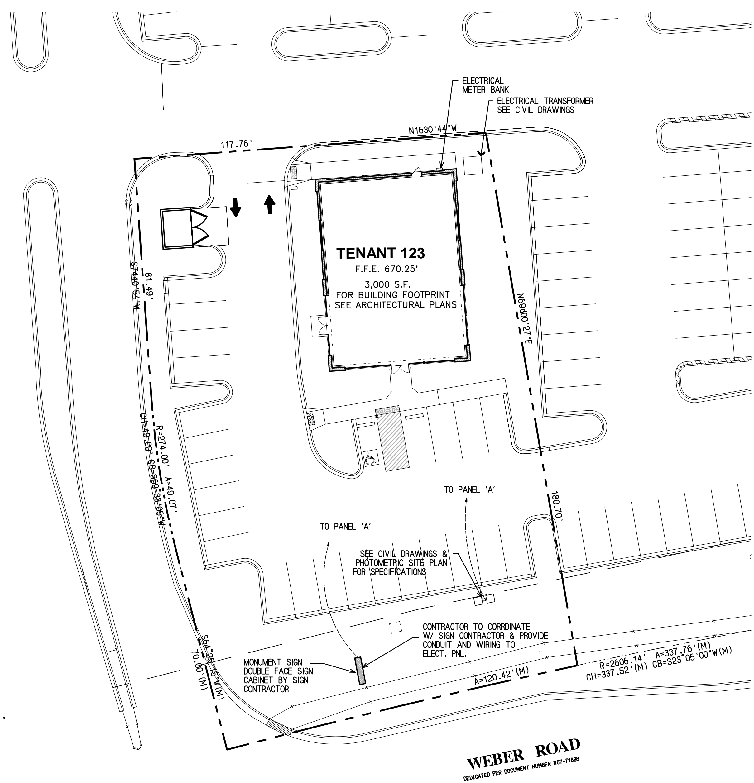
Site Electrical Plan SCALE: 1"=20'-0"
