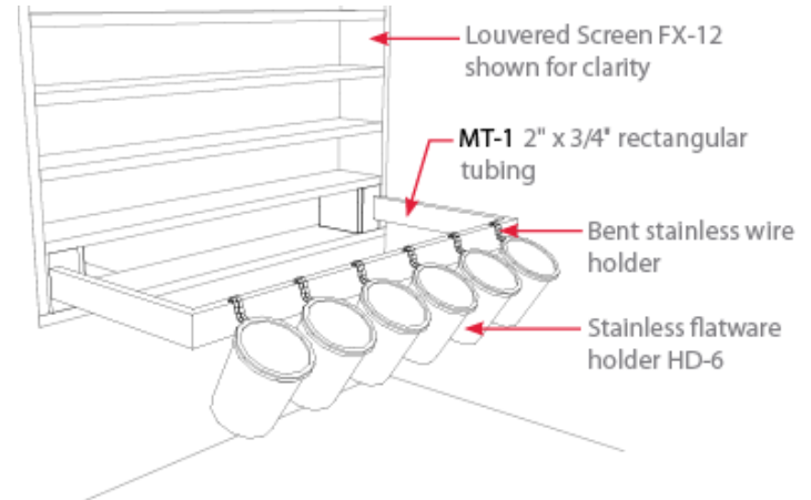
FX-10 Beverage Center Supply Rack
