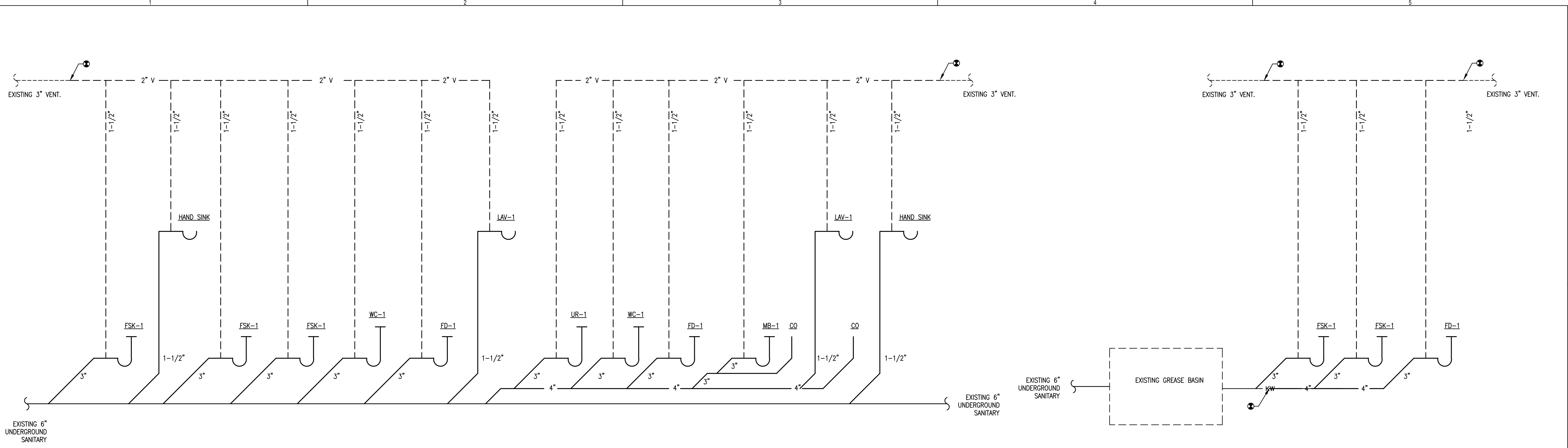
SANITARY WASTE RISER
