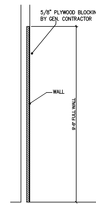
WALL BLOCKING DETAIL "G" NOT TO SCALE
