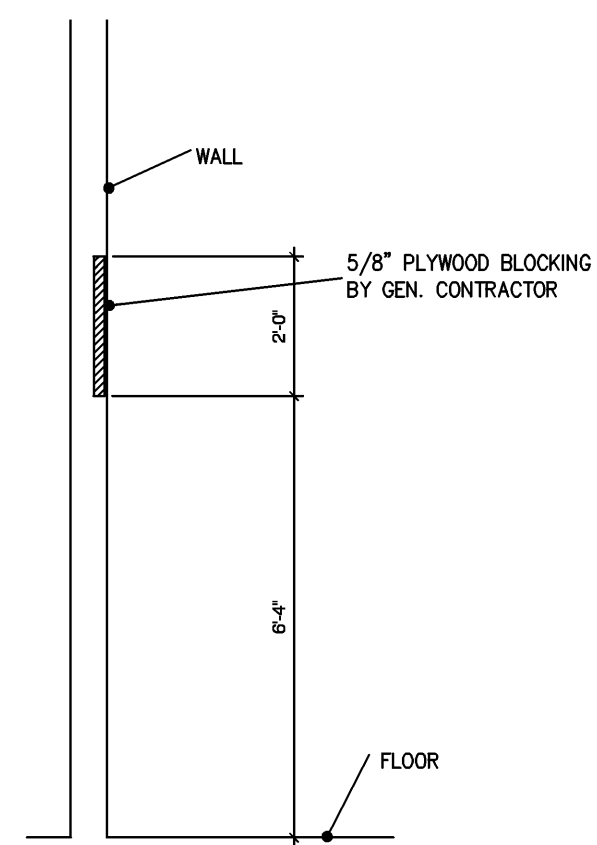
WALL BLOCKING DETAIL "B" NOT TO SCALE
