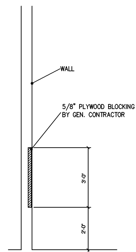
WALL BLOCKING DETAIL "E" NOT TO SCALE
