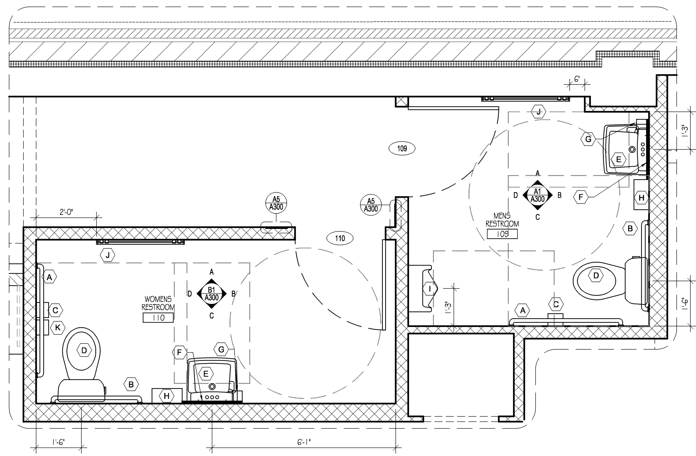
C1 ENLARGED RESTROOM PLAN Scale: 1/2" = 1'-0"
