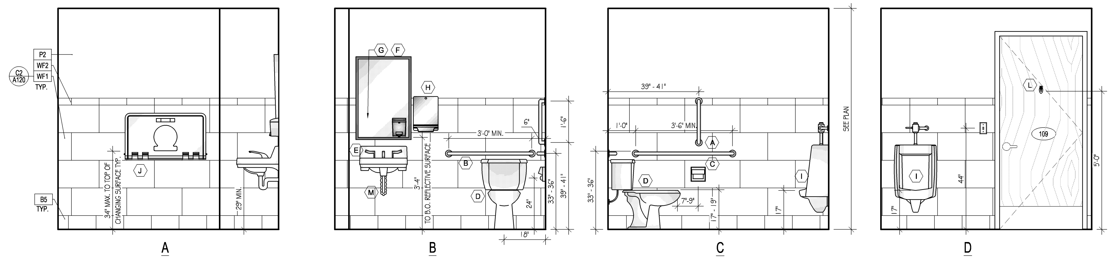
A1 MENS RESTROOM ELEVATIONS Scale: 1/2" = 1'-0"
