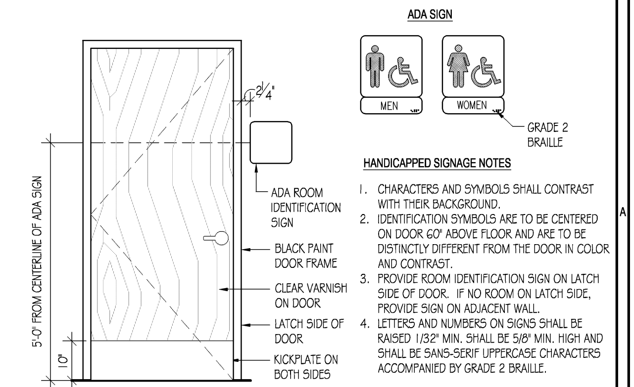
A5 RESTROOM SIGNAGE DETAIL Scale: 1/2" = 1'-0"
