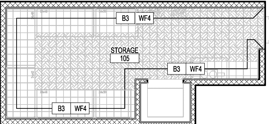
A120 STORAGE AREA FINISH PLAN Scale: 1/4" = 1'-0"
