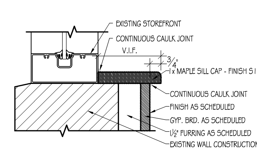
D3 TYPICAL WINDOW SILL DETAIL Scale: 3" = 1'-0"
