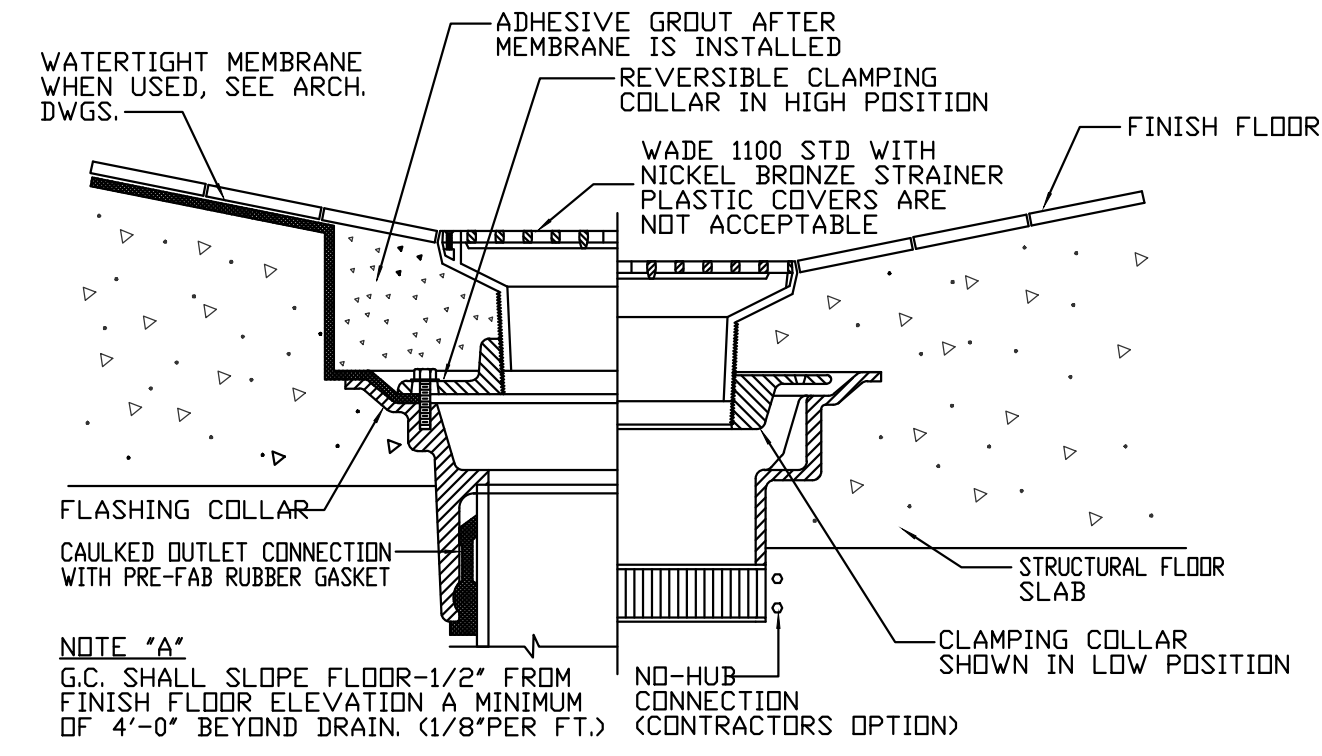
1 SLOPED FLOOR DRAIN DETAIL P1.2 SCALE: NONE
