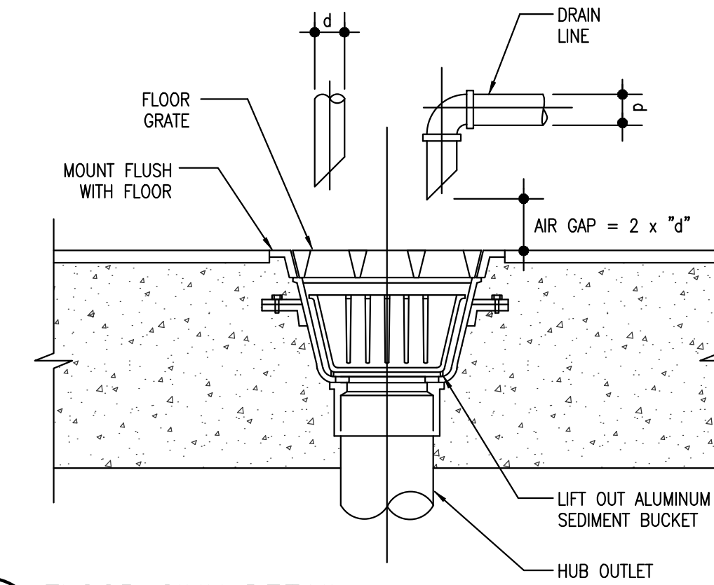
4 FLOOR SINK DETAIL P1.1 SCALE: NONE
