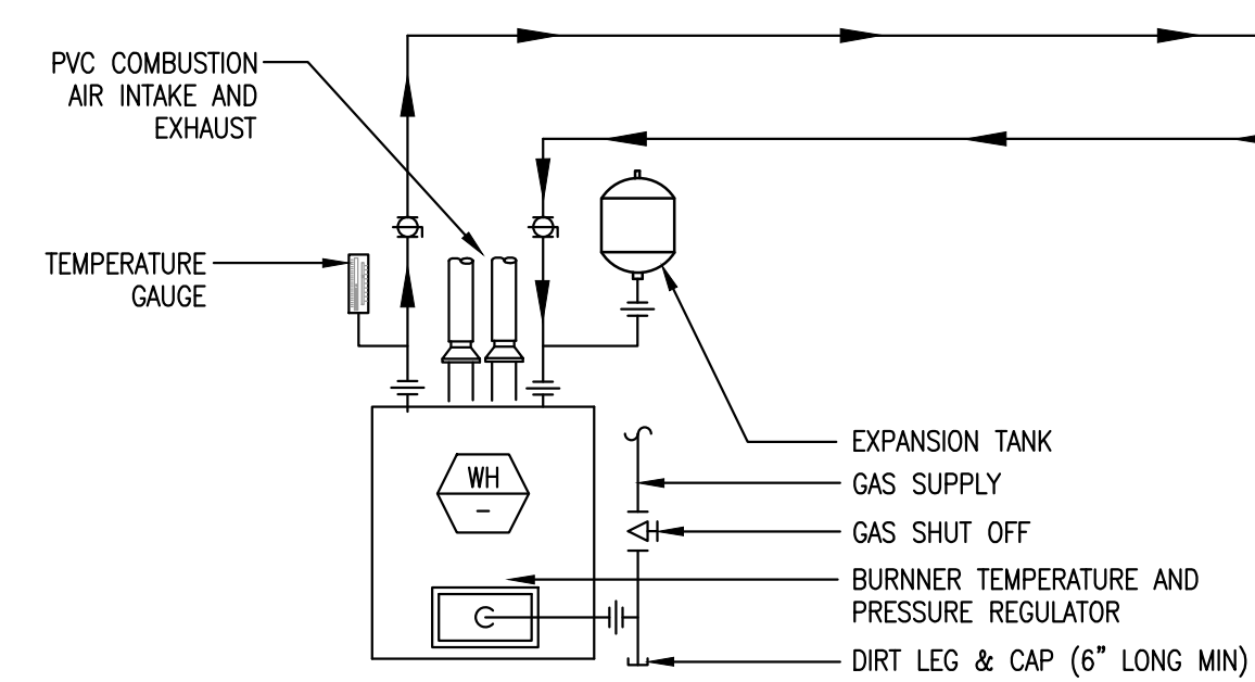
3 GAS INSTANTANEOUS WATER HEATER DETAIL P1.1 SCALE: NONE
