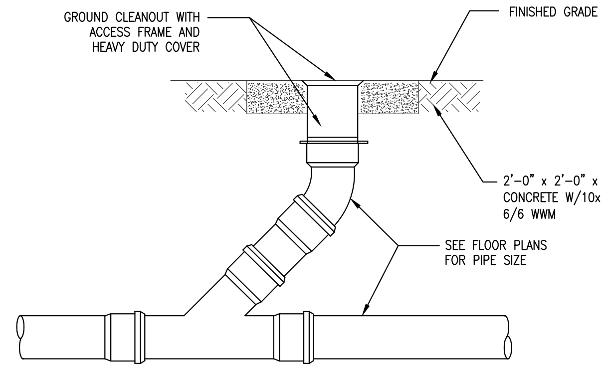
2 FLOOR CLEANOUT DETAIL P1.1 SCALE: NONE
