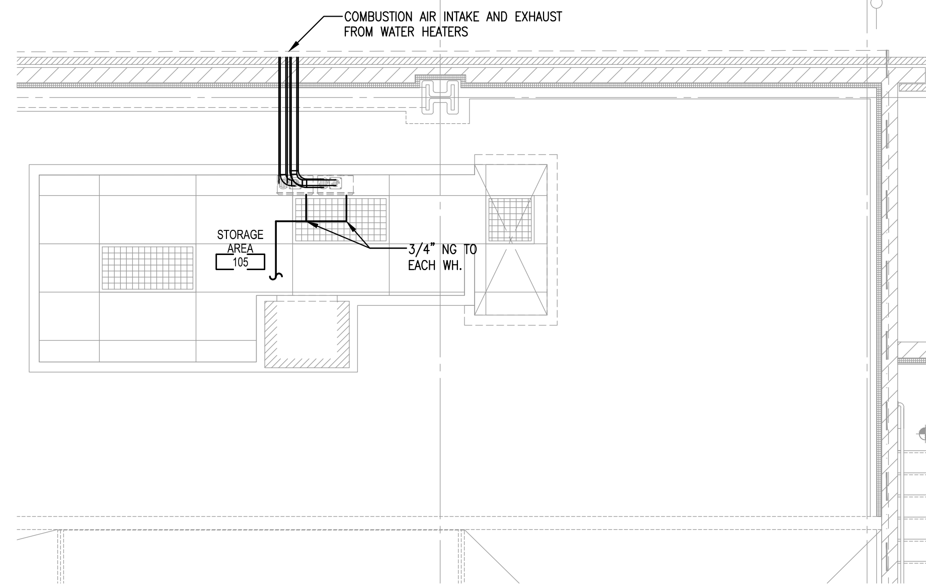
STORAGE AREA MECHANICAL PLAN
