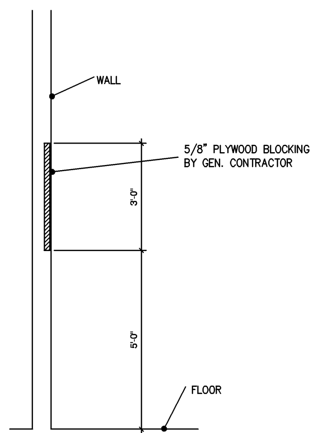
WALL BLOCKING DETAIL "C" NOT TO SCALE
