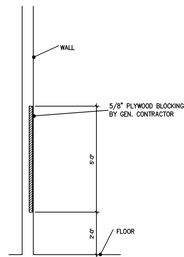
WALL BLOCKING DETAIL "A" NOT TO SCALE
