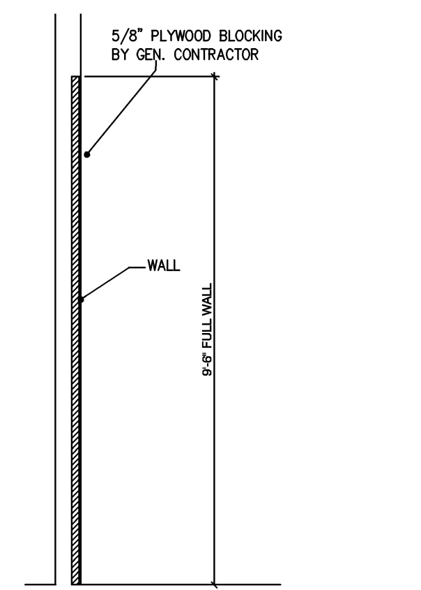
WALL BLOCKING DETAIL "G" NOT TO SCALE
