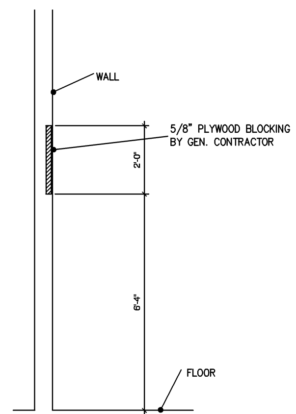
WALL BLOCKING DETAIL "B" NOT TO SCALE
