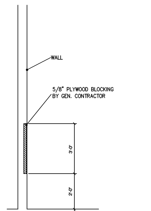
WALL BLOCKING DETAIL "E" NOT TO SCALE
