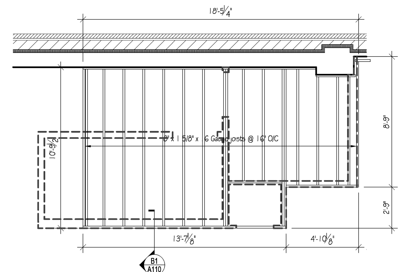
B2 STORAGE AREA FLOOR FRAMING PLAN
