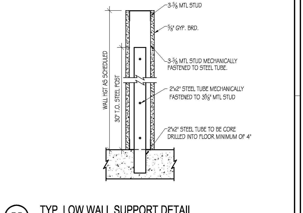
B5 TYP. LOW WALL SUPPORT DETAIL
