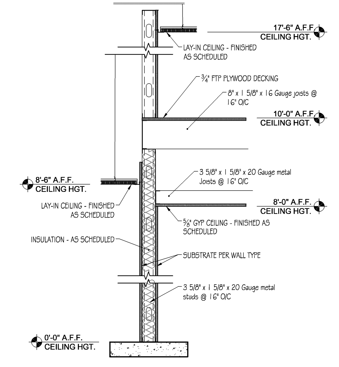
B1 WALL SECTION AT STORAGE AREA
