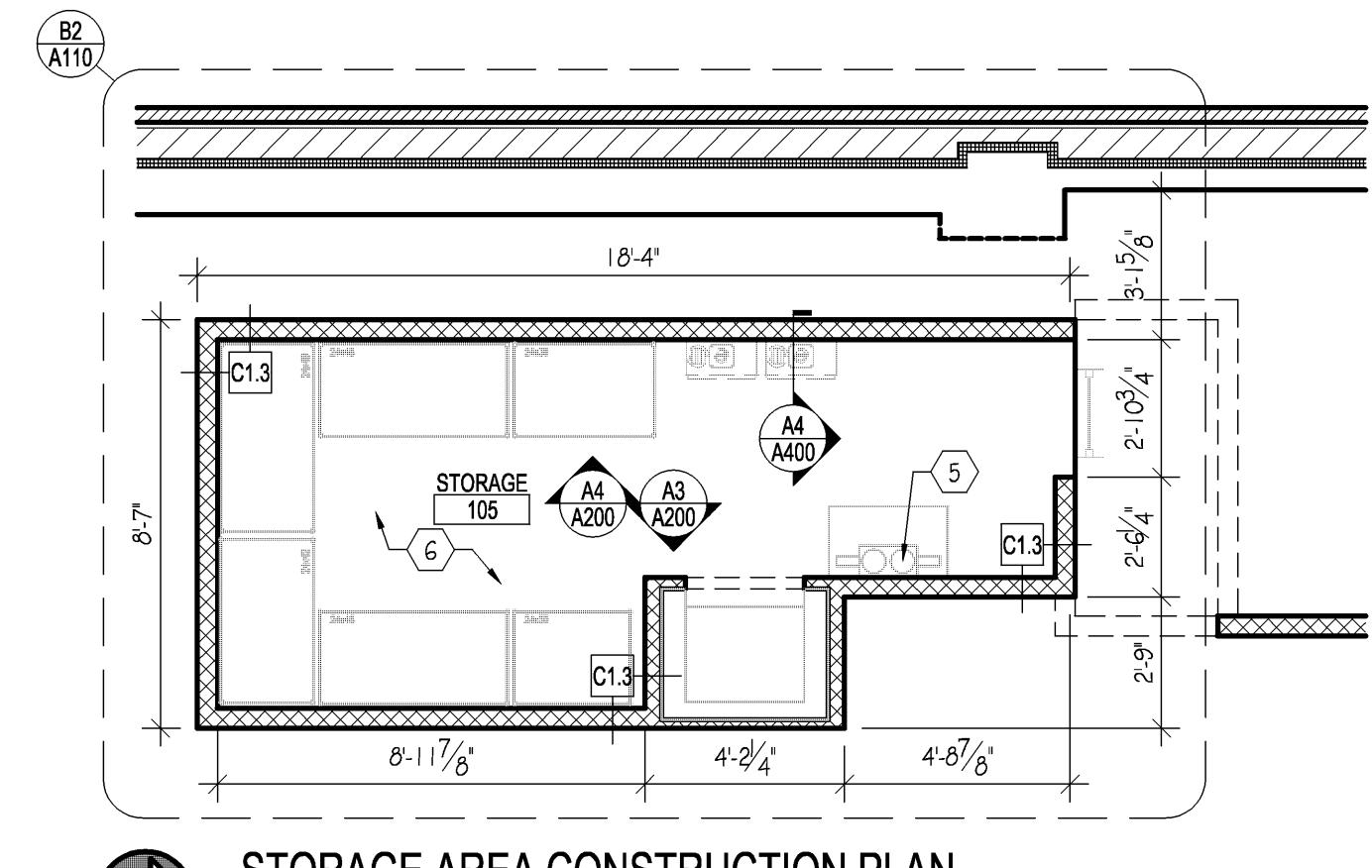
B3 STORAGE AREA CONSTRUCTION PLAN
